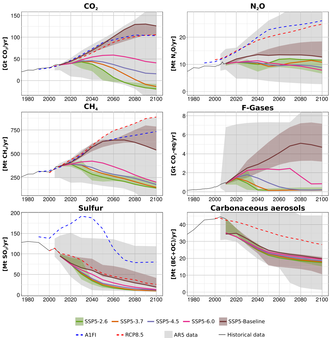
Fig. 9. Emissions of CO 2 , N 2 O, CH 4 , F-Gases, Sulfur and carbonaceous aerosols (OC+BC) for the SSP5 baseline and mitigation cases as derived by REMIND-MAGPIE. The SSP5 baseline emissions are compared with the emissions in the RCP8.5 and the A1FI marker scenario from SRES. Also shown are the funnels spanned by all SSP5 IAM interpretations for SSP5-Baseline and SSP5-2.6 (lighter colors) and the 5th to 95th percentile range of emissions scenarios in the AR5 scenario database. Differences in base year emissions are due to calibration to different data sources.
